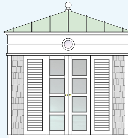
FRONT ELEVATION 10'W
